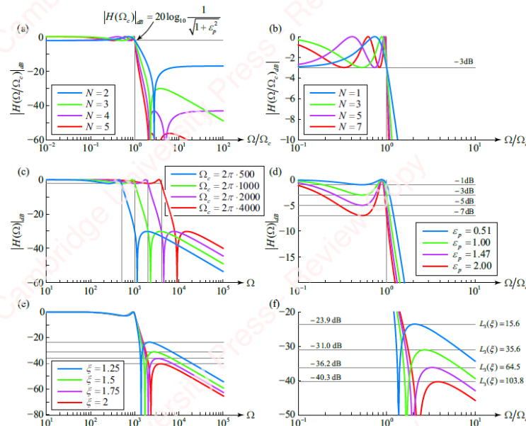
Figure 8.14 Dependence of elliptic filter on filter parameters N , \Omega_c , \epsilon_p and \zeta
